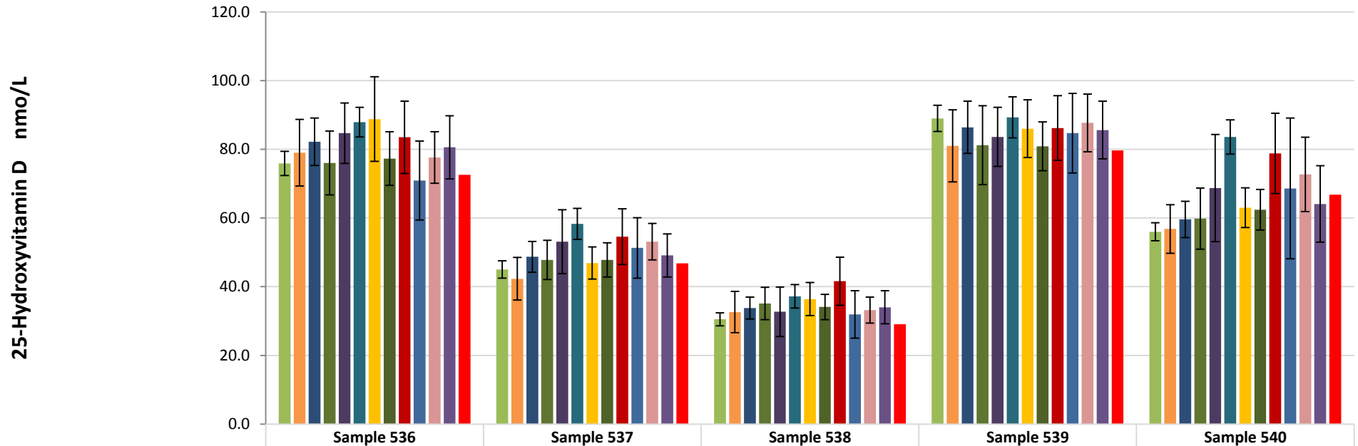
DEQAS July 2018 - 25-OHD Method Means (+/-1SD) for Major Method Groups*
